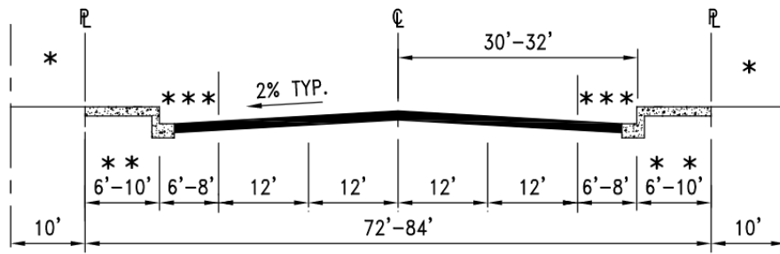
Figure 12: Existing Typical Section for Secondary Arterial (Commercial Street)
